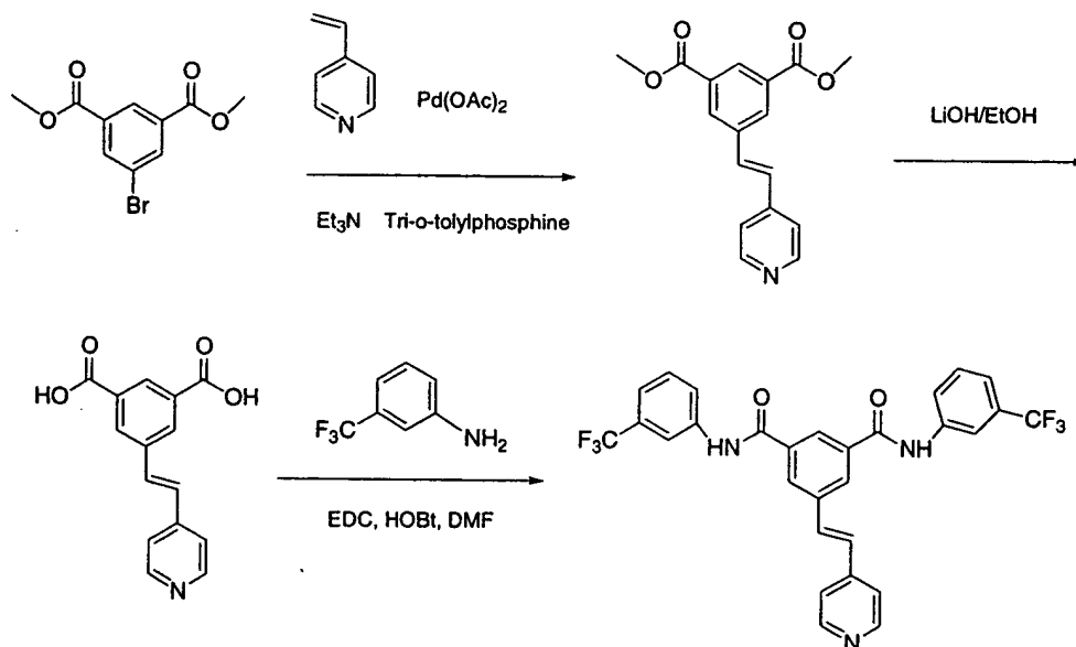
Scheme I-C
